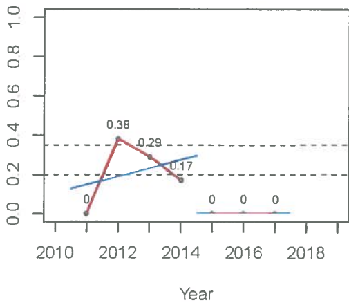
Success Rate Old Rule Ave: 0.21 Current Rule Ave: 0
