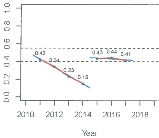
Success Rate Old Rule Ave: 0.29 Current Rule Ave: 0.43
