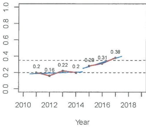
Success Rate Old Rule Ave: 0.2 Current Rule Ave: 0.32
