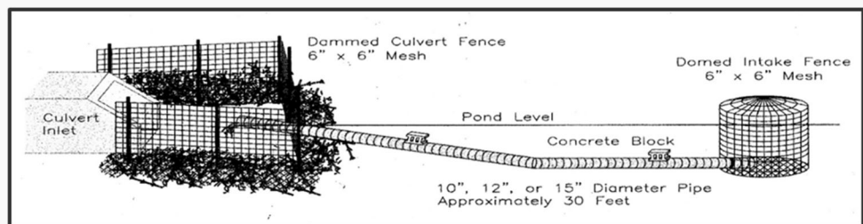
Fence-and-pipe system (photo left and diagram right) with a pipe running from above the obstruction and fencing to the culvert inlet downstream. P. Planer, RangeWorks LLC.
