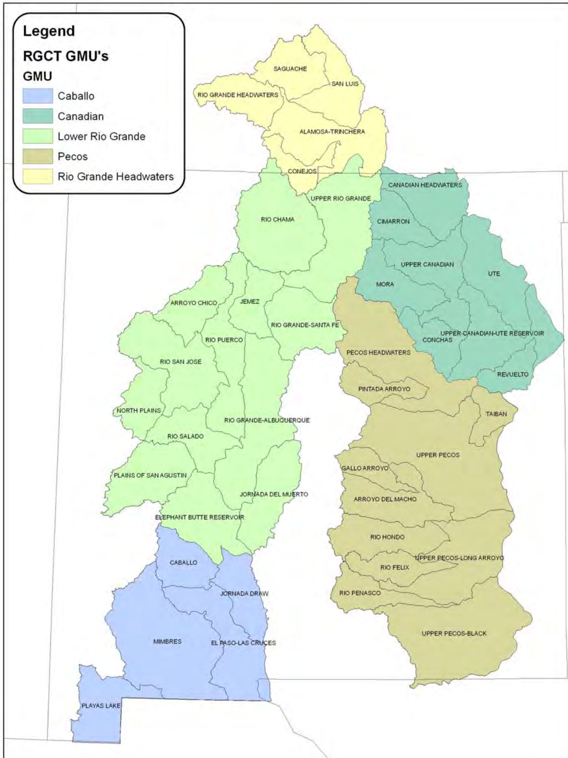
Figure 1. RGCT geographic management units based on second level hydrologic unit boundaries.
